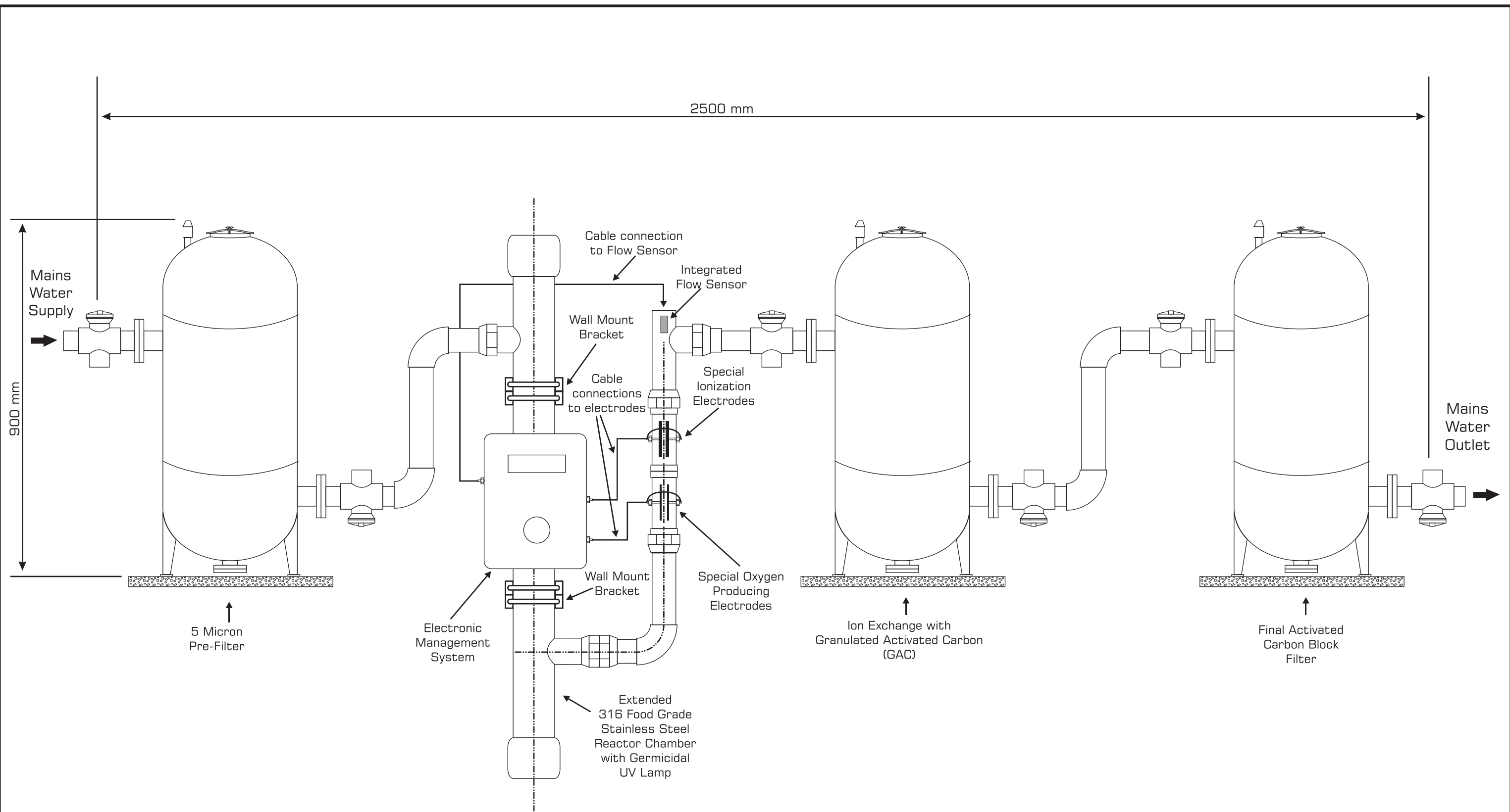
Schematic diagram ECO-CLEAR new generation series Whole House System
